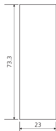
Door Cut-out Details
